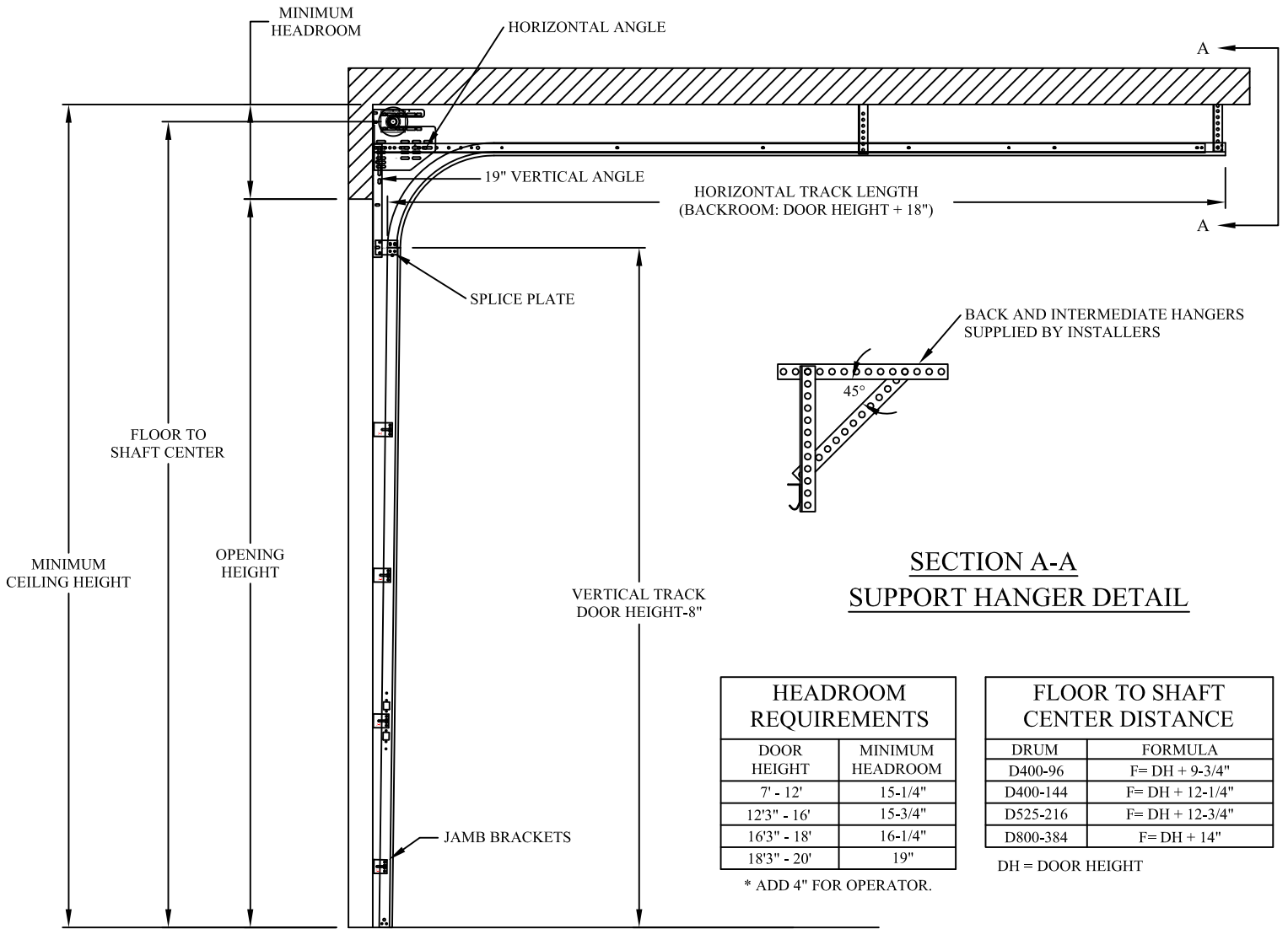
STANDARD LIFT BRACKET MOUNT TRACK SET DETAIL
